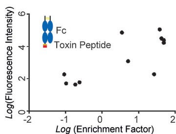
Figure 4. Correlation between Kv1.3 binding ability and enrichment factor. HEK293F cells transiently transfected with Kv1.3 were stained with the variants and analyzed with flow cytometry. The fluorescence intensities were plotted against the enrichment factors of the variants as calculated from NGS results.
